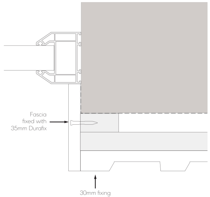
Fig. 14 - Window/door jamb with fascias
