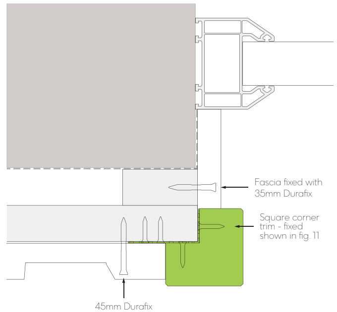
Fig. 12 - Window/door jamb with corner trim
