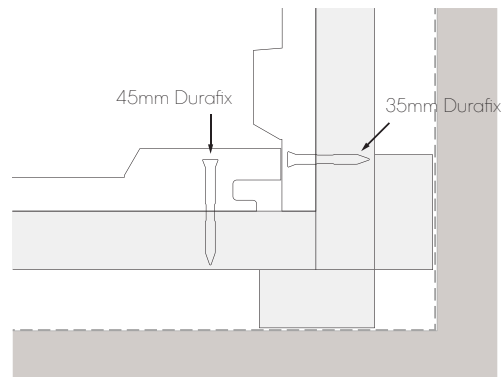
Fig. 9 - Internal mitred corner detail
