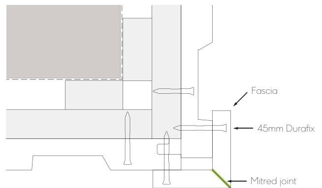
Fig. 10 - External mitred corner detail
