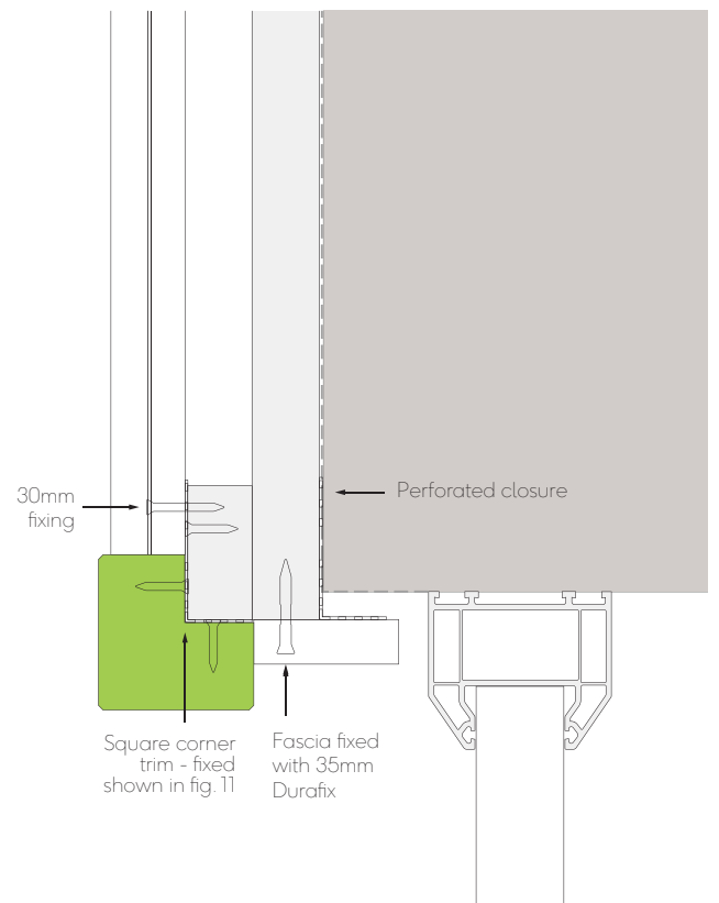
Fig. 13 - Window/door head with corner trim
